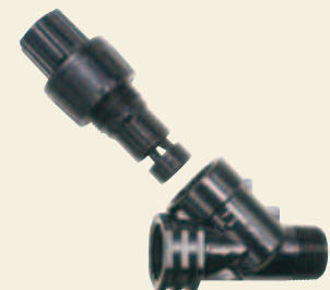
Exploded view of 3/4" High Flow Valve with replaceable Pressure Regulating module.
